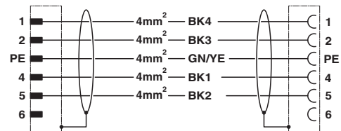
Contact assignment of M23 plugs/sockets
